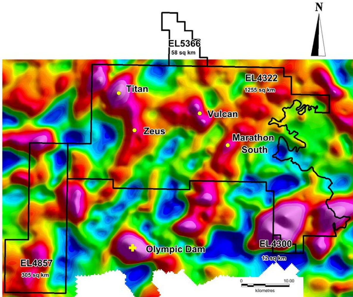
Figure 7: Lake Torrens Project Area Showing Main IOCGU Targets Over Residual Gravity Image
