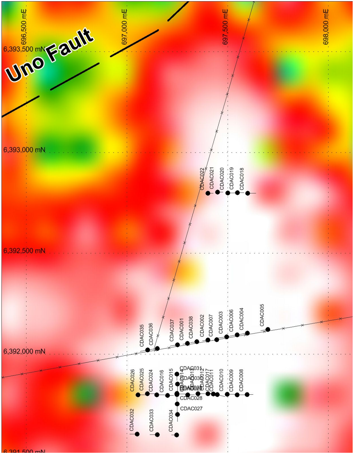
Figure 6: Corrie Dam prospect, drill hole location plan showing surface projections of inclined hole traces over portion of Ag soil anomaly image.
