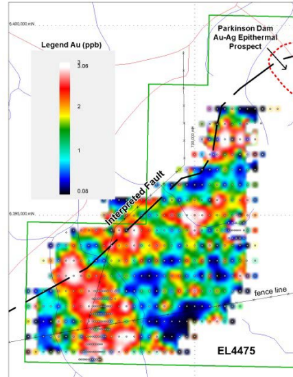
Figure 5b: Corrie Dam Gold Image
