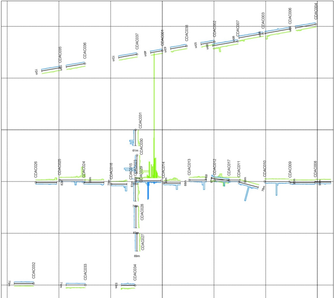
Figure 7: Corrie Dam prospect, plan of southern drill hole locations showing Pb (green) and Ag (blue) bar graphs on 100m grid spacing. Highest Pb and Ag values in hole 15 inclined to east.
