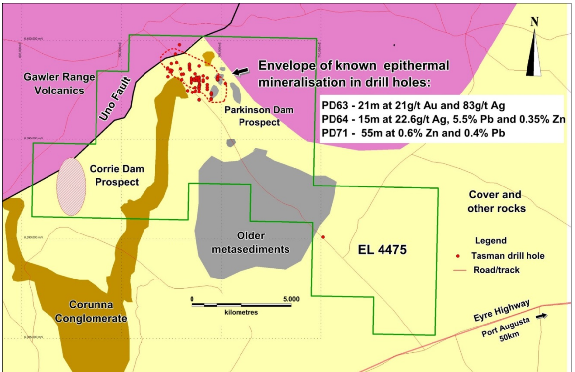
Figure 2: Plan of Tasman's Parkinson Dam prospect (now EL 5602, previously EL4475) showing area of previously defined epithermal mineralisation and recently discovered Corrie Dam prospect adjacent to the Gawler Range Volcanics. (GDA 94; Zone 53).
